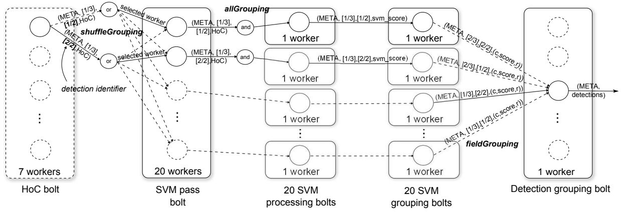
Figure 3: The overview of the last step containing SVM related bolts.
