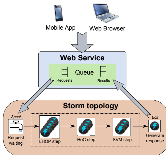
Figure 1: An overview of the system with front-end web-service and back-end implementation of the object detection on a distributed processing platform.
